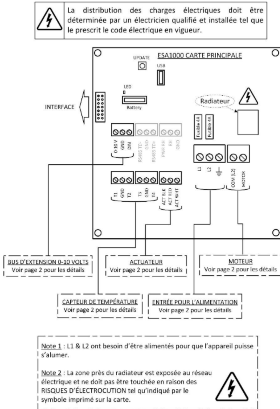
FIGURE 2: WIRING DIAGRAM
